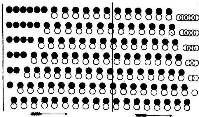
MIGRATION OF THE IONS ACCORDING TO HITTORF
